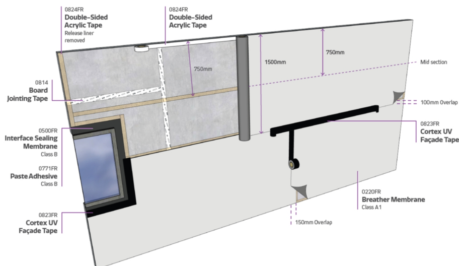
Diagram 1 - Typical wall construction
